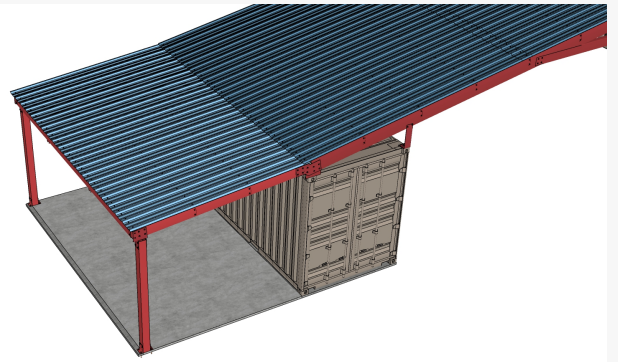
Gable 56' span with awning
